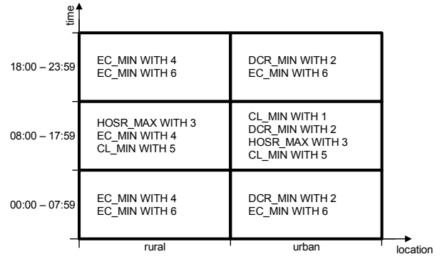
Figure 4. KPI target-priority-state space example (CL_MIN refers to minimization of the cell load, DCR_MIN refers to minimization of the dropped call rate, EC_MIN refers to minimization of the energy consumption, HOSR_MAX refers to maximization of the handover success rate)
