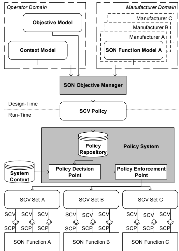
Figure 2. Overview of the SON Objective Manager and Policy System
