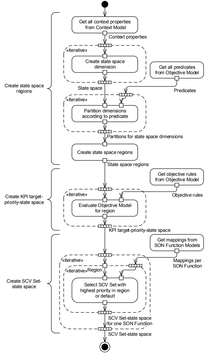
Figure 3. SCV Policy derivation algorithm (noted in UML 2)
