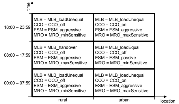
Figure 5. SCV Set-state space example
