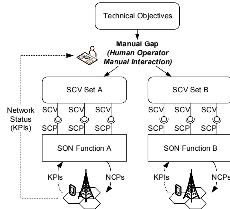
Figure 1. Manual gap between technical objectives and SCV Sets (NCP refers to networks configuration parameter)
